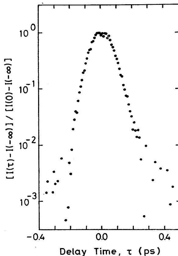
FIG. 7. Normalized signal intensity as a function of delay time in nitrobenzene at 553 nm. The polarization configuration is type II.
