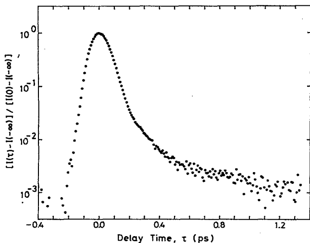
FIG. 3. Normalized signal intensity as a function of delay time in CS 2 at 553 nm. Polarization configuration is type I.
