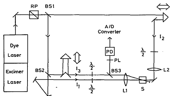
FIG. 1. Experimental setup for the degenerate four-wave mixing using incoherent light. BS1 and BS2 are the beam splitters; BS3, the glass plate; L1, L2, the lens; PD, the photodiode; PL, the polarizer; RP, the Rochon prism; S, the sample; \lambda/2 , the half-wave retarder.
