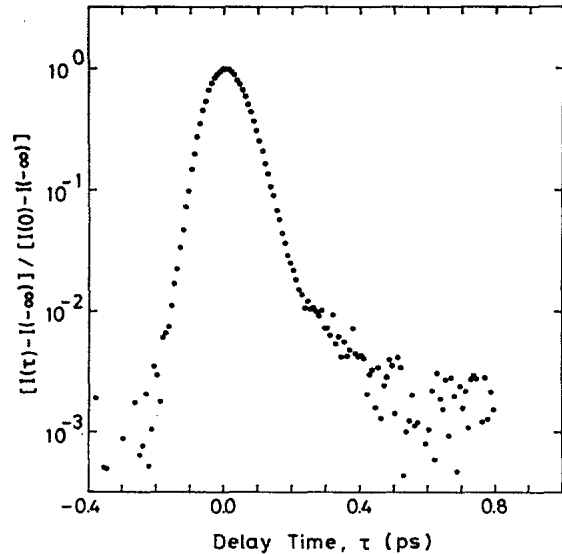
FIG. 4. Normalized signal intensity as a function of delay time in CS 2 at 553 nm. Polarization configuration is type II.
