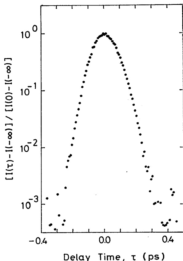
FIG. 6. Normalized signal intensity as a function of delay time in nitrobenzene at 553 nm. The polarization configuration is type I.
