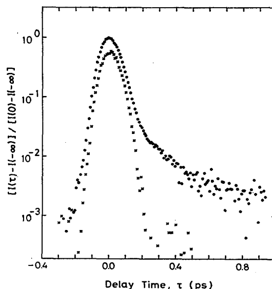
FIG. 2. Normalized signal intensity as a function of delay time \tau of I_1 to I_3 . Signal intensity is normalized by the difference between the intensity at \tau=0 , I_s(0) , and the intensity at \tau=-\infty , I_s(-\infty) . (●), CS 2 in type-I polarization configuration, where I_3 is vertically polarized and both I_1 and I_2 are horizontally polarized. (×), reference sample (DEANS in CS 2 ) in type-II polarization configuration, where I_1 , I_2 , and I_3 are all vertically polarized. The wavelength is 553 nm. Plot of the normalized signal intensity in reference sample is slightly shifted down.
