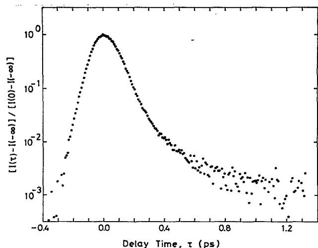
FIG. 5. Normalized signal intensity as a function of delay time in CS 2 at 623 nm. Polarization configuration is type I.
